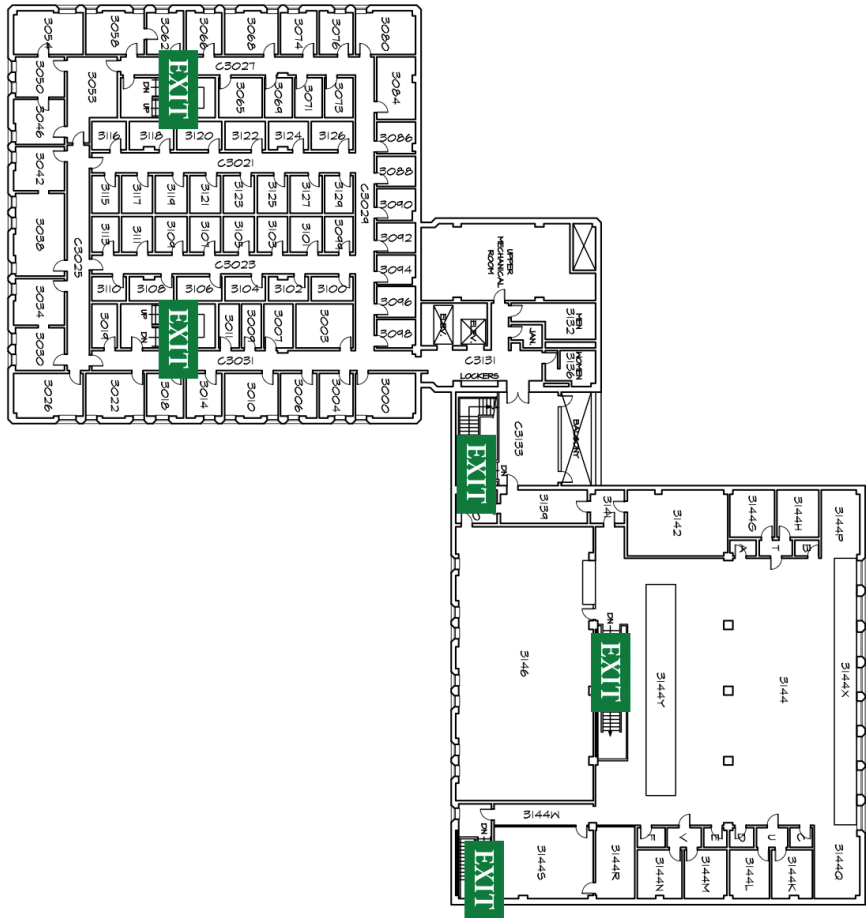
NORTH 0 16 32 48 64 FEET THIRD FLOOR PLAN
