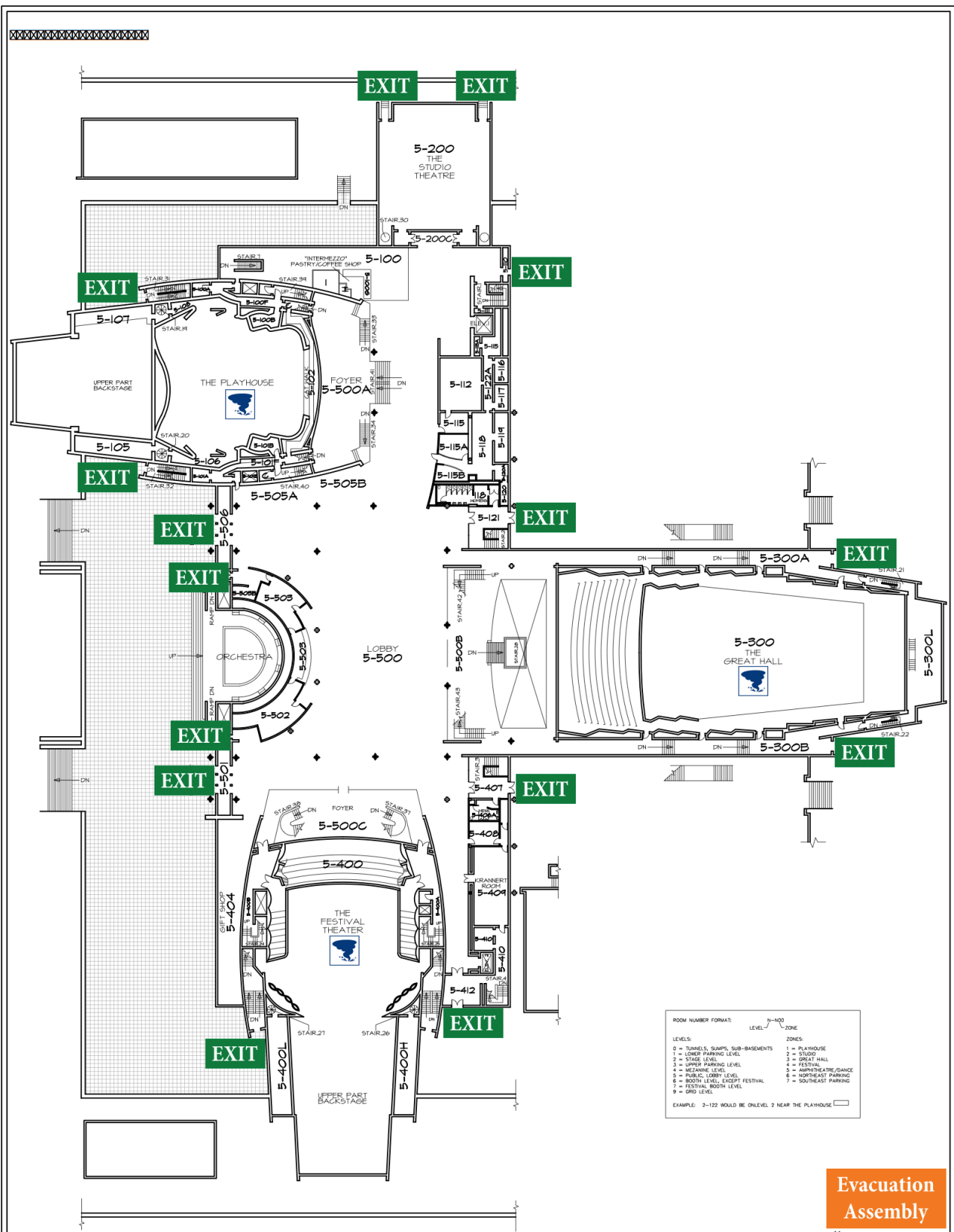
PUBLIC/LOBBY LEVEL PLAN NORTH 0 32 64 96 128 FEET
