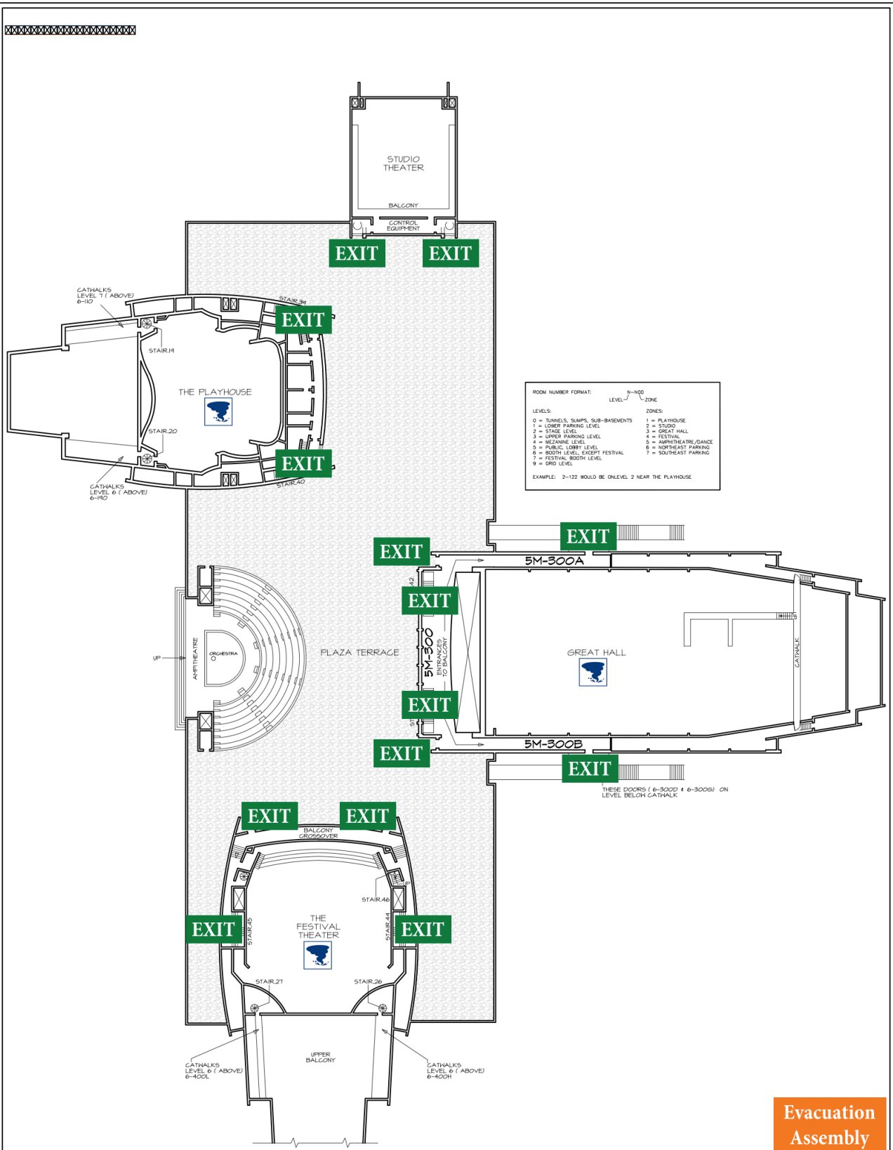
NORTH FIFTH MEZZANINE PLAN 0 32 64 96 128 FEET
