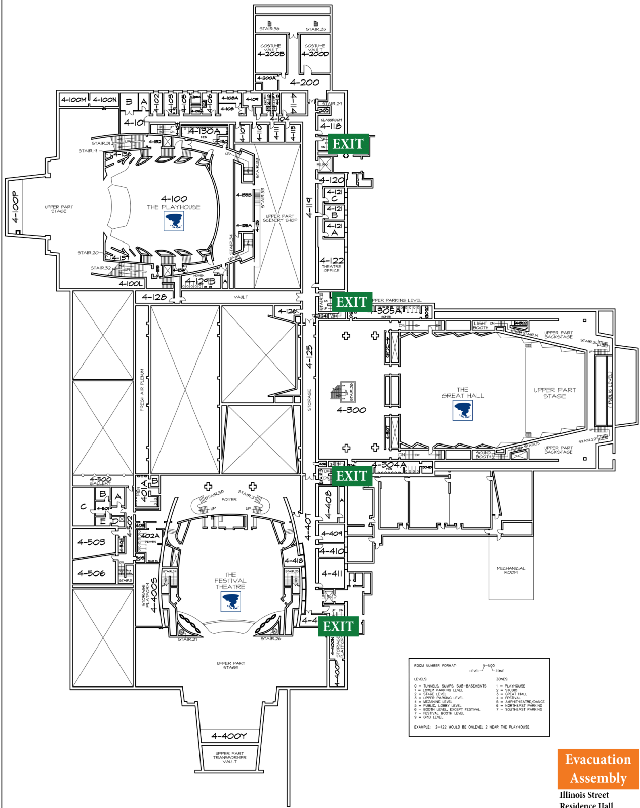
NORTH MEZZANINE LEVEL PLAN 0 32 64 96 128 FEET
