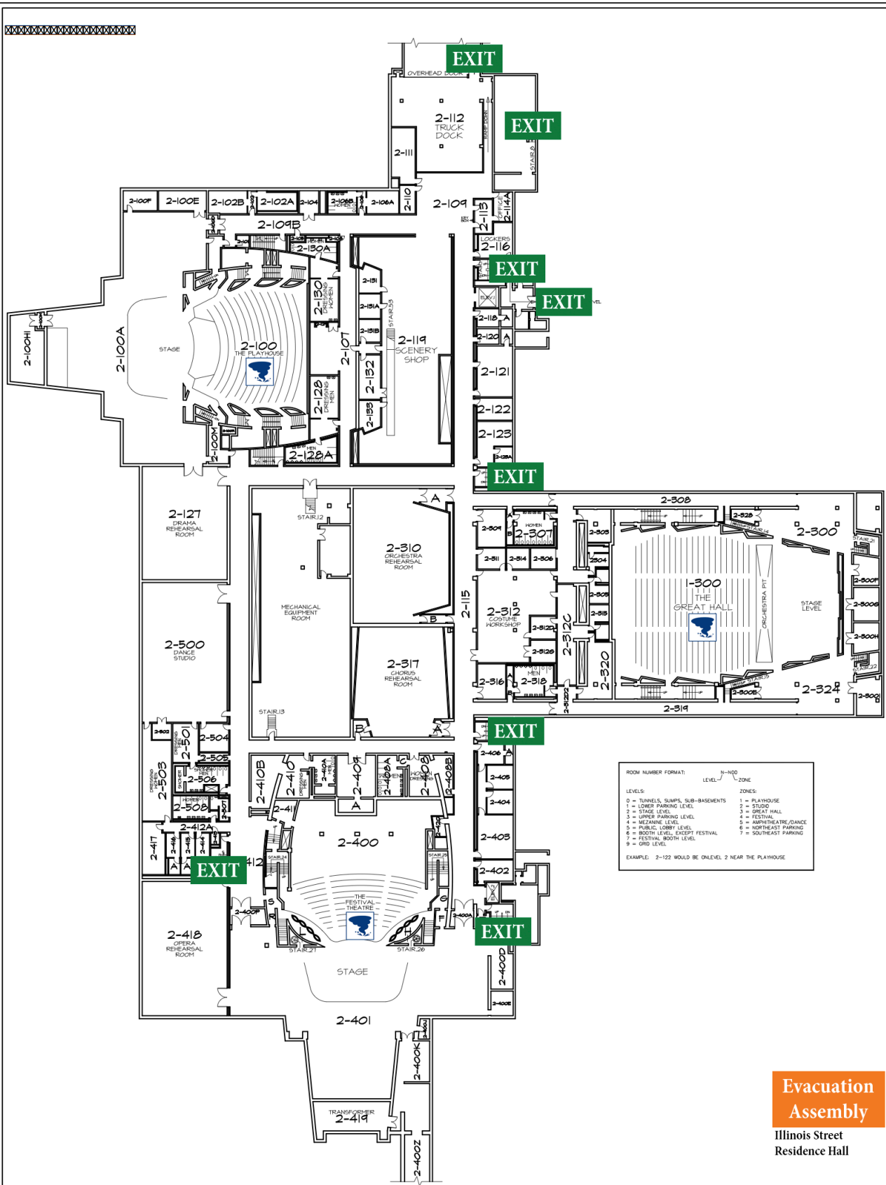
NORTH STAGE LEVEL PLAN 0 32 64 96 128 FEET
